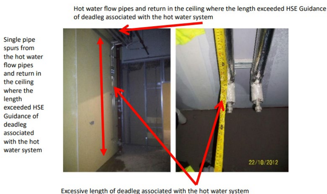
Figure 2. Excessive length of deadleg associated with hot water system.
